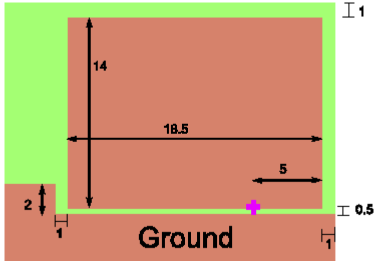
Figure 26. Patch Antenna 1
