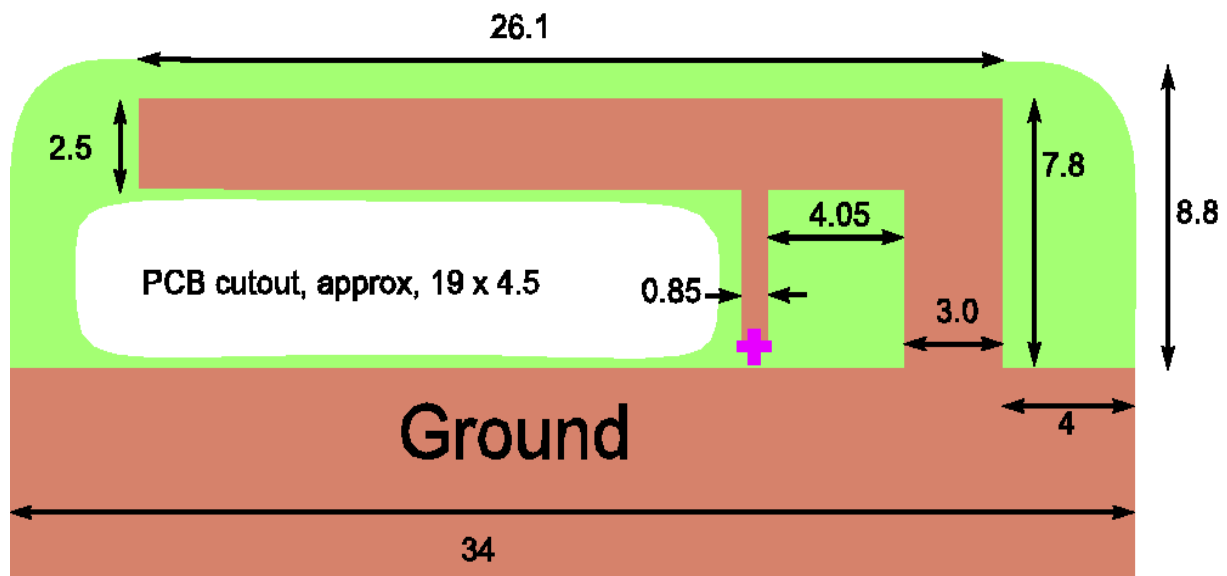
Figure 12. F Antenna 2
