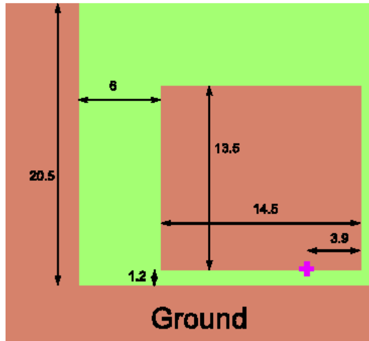
Figure 27. Patch Antenna 2
